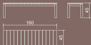
VINTAGE bench 160 cm
