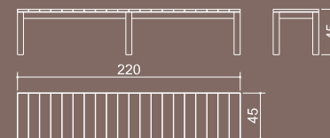
VINTAGE bench 220 cm
