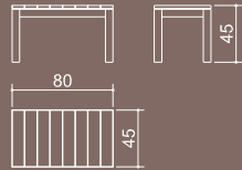
VINTAGE bench 80 cm
