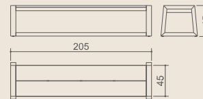
BAIA bench 205 cm Code: MG 5202 Materials : aluminum, recycled teak Optional cushion Sunbrella: MG 8043-sbr Optional cushion Stamskin: MG 8043-stm
