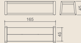
BAIA bench 165 cm Code: MG 5201 Materials : aluminum, recycled teak Optional cushion Sunbrella: MG 8043-sbr Optional cushion Stamskin: MG 8043-stm
