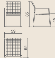
BAIA carver chair Code: MG 5200 Materials: aluminum, batyline
