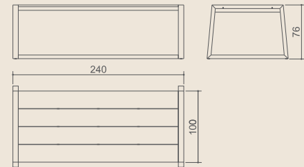
BAIA table 240x100 cm Code: MG 5204 Materials: aluminum, recycled teak Note: knock down - assembly required
