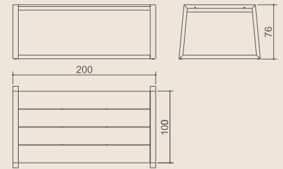
BAIA table 200x100 cm Code: MG 5203 Materials: aluminum, recycled teak Note: knock down - assembly required
